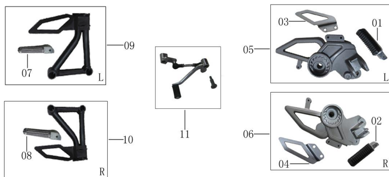
F-17 搁脚组合 FOOTRESTS
